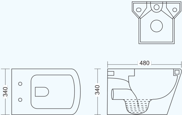
GI-302 WALL HUNG L 480 W 340 H 340mm
