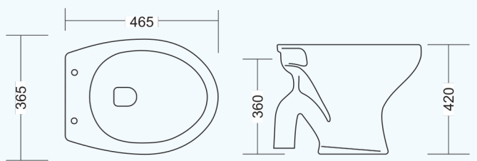
GI-402 EUROPEAN WATER CLOSET
