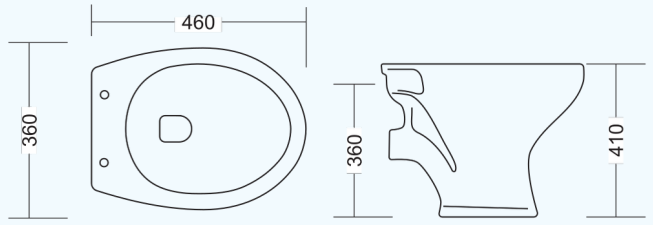
GI-401 EUROPEAN WATER CLOSET
