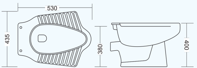
GI-403 ANGLO INDIAN WATER CLOSET
