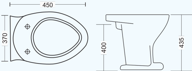
GI-406 RAILWAY WATER CLOSET (HOPPER)
