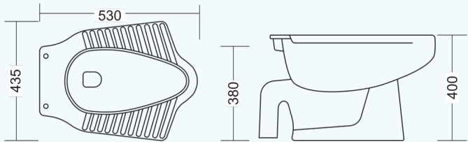
GI-404 ANGLO INDIAN WATER CLOSET
