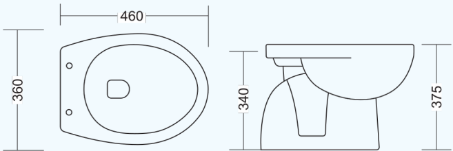
GI-405 CONCEALED WATER CLOSET
