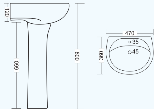
GI-502 18" x 14" MINI REPOSE SET L 360 W 470 H 800mm
